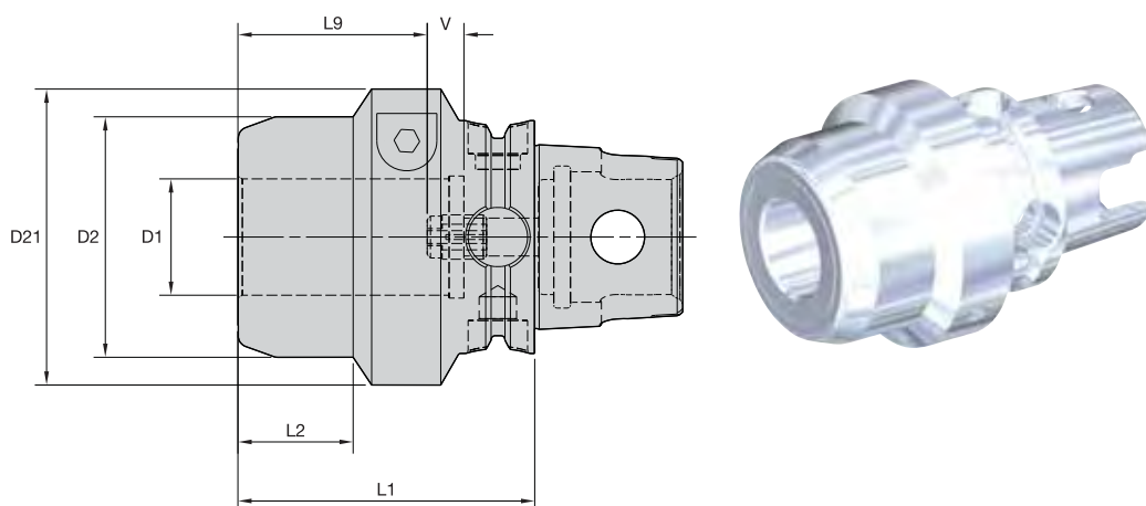
Cutting Tool Shank Requirements metric (ISO standard)
